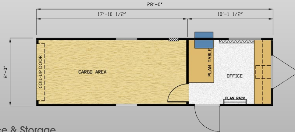
Do-All Mobile Office & Storage
